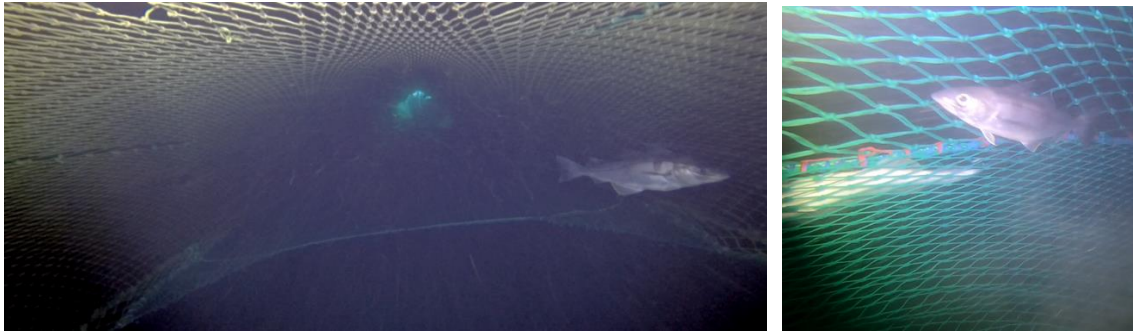
Fig. 9. Photo left side: The front of the vertical panel with a haddock on the “correct side” in the two-level trawl. Photo right side: Haddock and cod on correct side as entering the codends.
